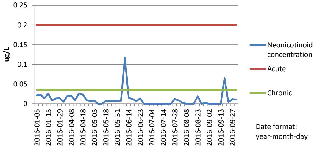
Figure 9 - Neonicotinoid Pollution in the River Ouse at Nether Poppleton (2016) - showing chronic and acute toxicity limits
