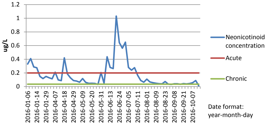
Figure 6 - Neonicotinoid Pollution in the River Waveney (2016) - showing chronic and acute toxicity limits
