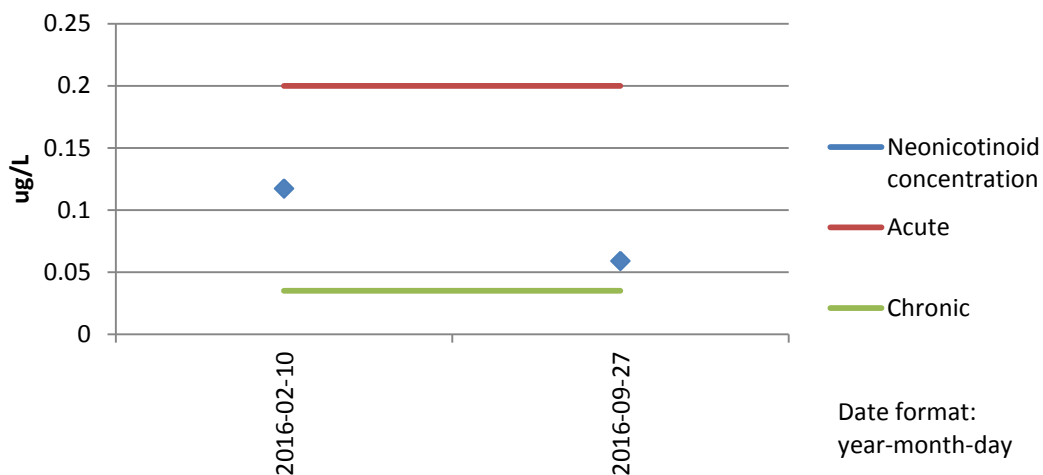
Figure 13 - Neonicotinoid Pollution at Sincil Dyke (2016) - showing chronic and acute toxicity limits
