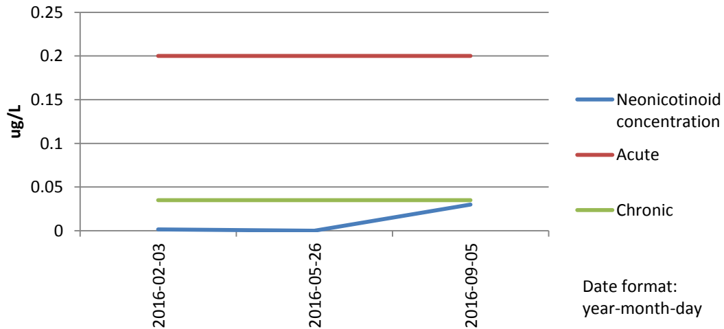
Figure 8 - Neonicotinoid Pollution in the River Chelt (2016) - showing chronic and acute toxicity limits
