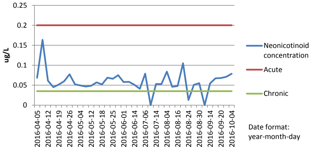
Figure 10 - Neonicotinoid Pollution in the River Ouse at Roxton Lock (2016) - showing chronic and acute toxicity limits
