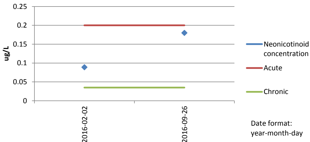
Figure 14 - Neonicotinoid Pollution at Somerhill Stream (2016) - showing chronic and acute toxicity limits
