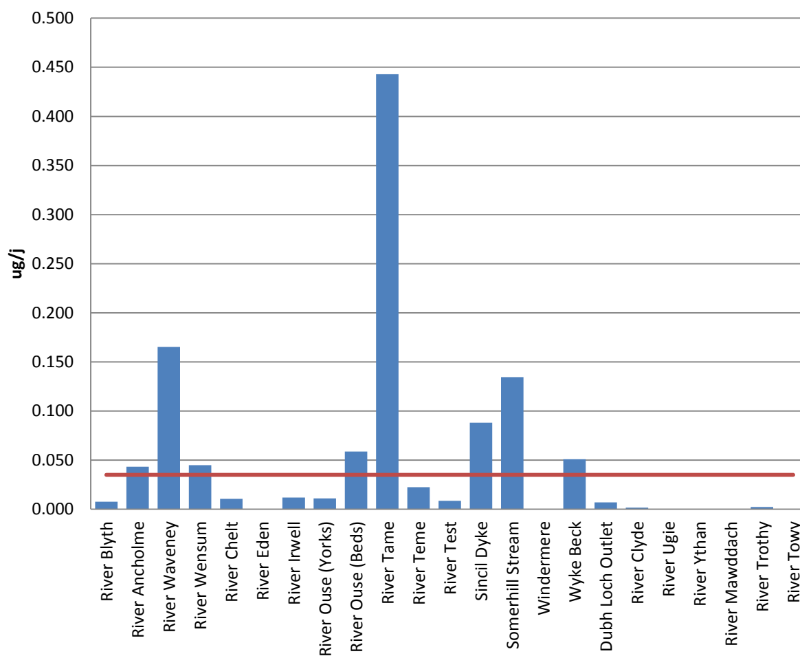
Figure 21 - Average Annual Neonicotinoid Concentration
