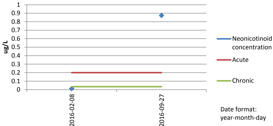
Figure 11 - Neonicotinoid Pollution in the River Tame (2016) - showing chronic and acute toxicity limits
