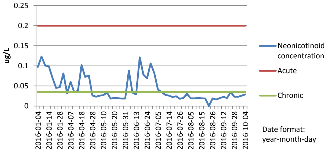
Figure 7 - Neonicotinoid Pollution in the River Wensum (2016) - showing chronic and acute toxicity limits
