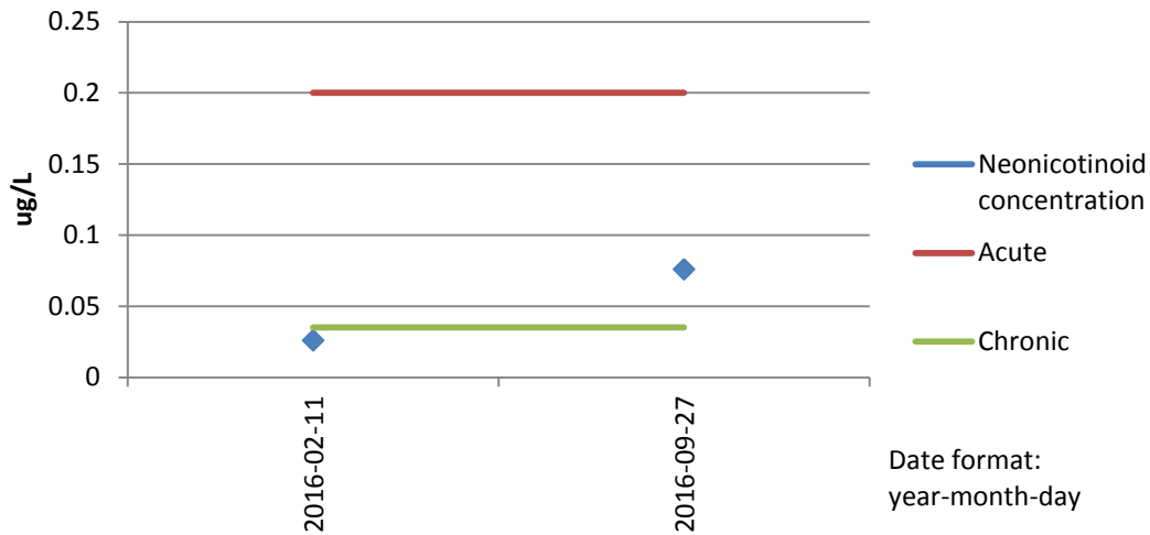
Figure 15 - Neonicotinoid Pollution at Wyke Beck (2016) - showing chronic and acute toxicity limits
