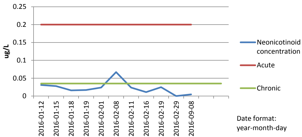
Figure 12 - Neonicotinoid Pollution in the River Teme (2016) - showing chronic and acute toxicity limits
