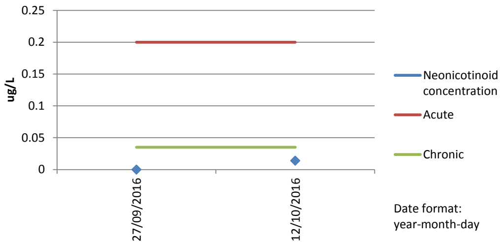
Figure 17 - Neonicotinoid Pollution at Allt an Dubh Loch (2016) - showing chronic and acute toxicity limits
